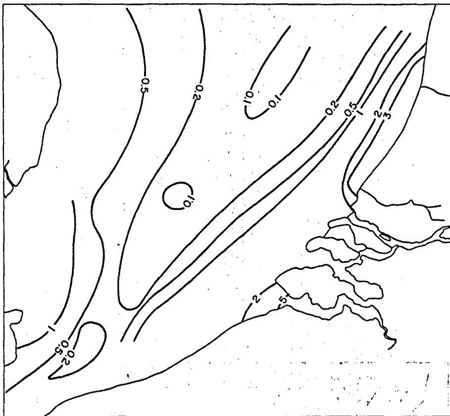
Figure 2b. Sol. PO4-P, 10^{-6} M Surface 1-5 Oct. 1973
