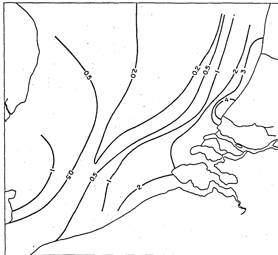
Figure 2c. Sol. PO4-P, 10^{-6} M Surface 29 Oct.-1 Nov. 1973
